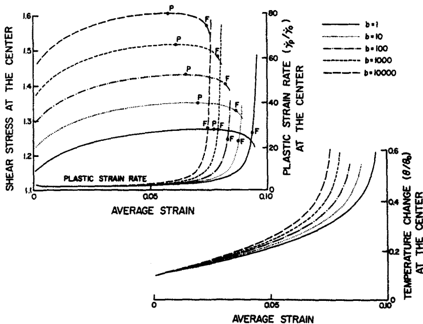
Fig. 1. Effect of the value of material parameter b on the evolution of the central stress, central plastic strain rate and the central temperature.
