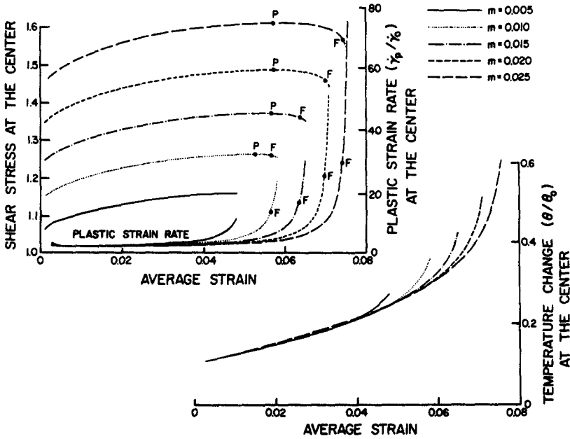
Fig. 3. Stress-strain curves and the evolution of the central plastic strain rate and temperature for different values of m .
