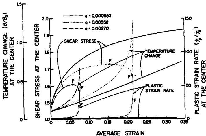
Fig. 7. Effect of the value of the thermal softening coefficient a on the growth of the central stress, plastic strain rate and temperature.
