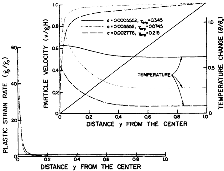
Fig. 8. Variation of the particle velocity, temperature and plastic strain rate within the specimen for different values of a .
